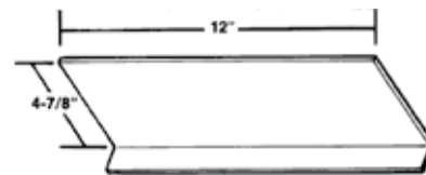
STIFFENER PLATE Part No. P2056M
