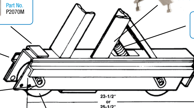
WHEEL Part No. P0310M 2-1/2" X 7/8" X 1/4"
