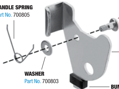
HANDLE LATCH Part No. 856179
